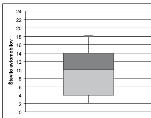
Excel 2007
