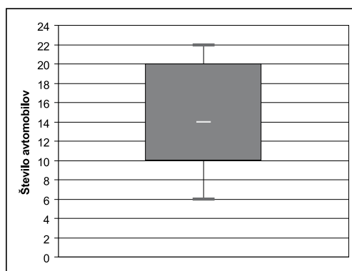
Excel 2003
